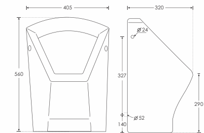
FLUID Urinal - 50006 L320 W405 H560mm
