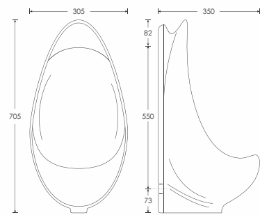
ANTEA Urinal - 50001 L350 W305 H705mm
