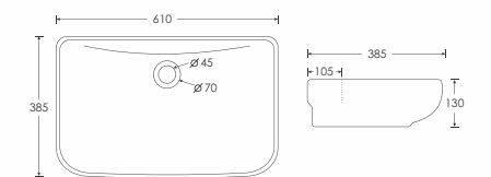
DB - 4001 Hand Crafted Basin L610 W385 H130mm
