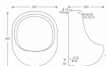
STAMEN Urinal - 50008 L322 W250 H390mm
