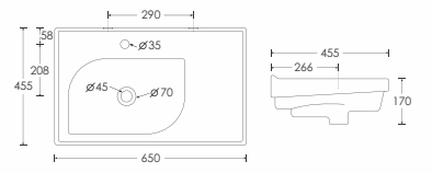
LEFT MINI SCENERY Wall Mounted Basin - 10106L L650 W455 H170mm
