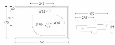
RIGHT SCENERY Wall Mounted Basin - 10104R L765 W470 H195mm
