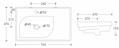
LEFT SCENERY Wall Mounted Basin - 10104L L765 W470 H195mm
