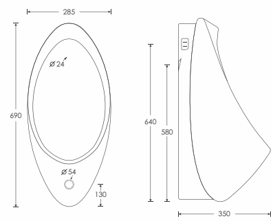
SAVVY Urinal - 50002 L350 W285 H690mm
