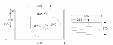
RIGHT MINI SCENERY Wall Mounted Basin - 10106R L650 W455 H170mm
