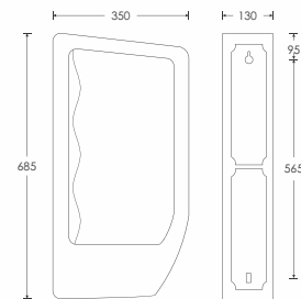
SLAT Divisional Plate - 50005 L350 W130 H685mm
