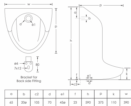
SCLUPTURE Urinal - 50003 (ISI) L375 W390 H590mm
