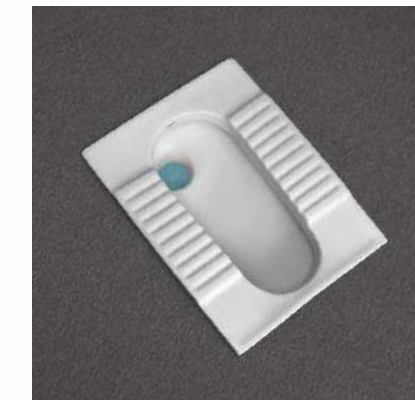
ORISSA 21" BR/OR Squatting Pan - 70001BR/OR L540 W425 H290mm
