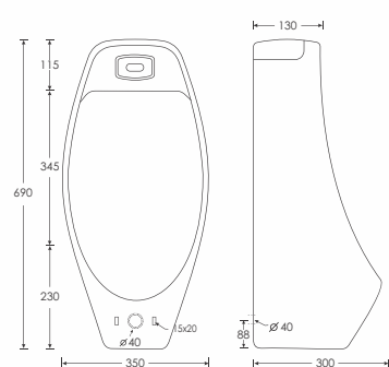
KELOS Urinal with Sensor - 52005 L350 W300 H690mm
